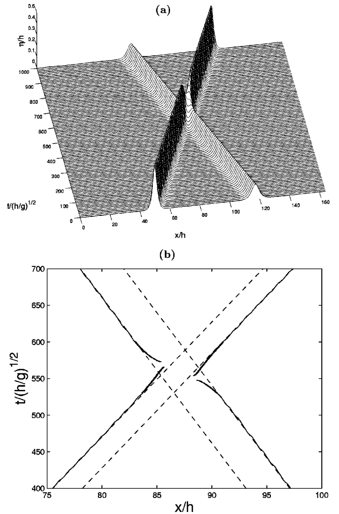
FIG. 15. Overtaking collision of two solitary waves of height S_1/h=0.4 , S_2/h=0.1333 : (a) (x,t) plot and (b) crest trajectory. The amplitudes after collision are S_1^+/h=0.4001 , S_2^+/h=0.1332 at t/\sqrt{h/g}=1000 for the large and small wave, respectively. The phase shifts are (a_1^+-a_1)/h=2.7424 and (a_2^+-a_2)/h=4.0591 , respectively.
