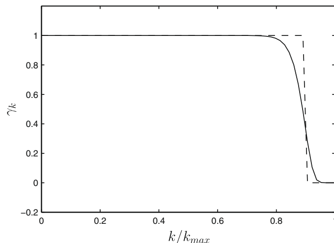
Fig. 1. Two-dimensional profiles of the ideal filter (28) with v = 0.9 , in dashed line, and Hou and Li's [35] exponential filter (29), in solid line.
